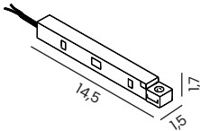
DRIVER OUTSIDE MEANWELL REGULAR (100W, 200W, 350W) Power/Code 100W ... AZ4691 200W ... AZ4692 350W ... AZ4866
