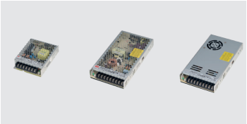
DRIVER OUTSIDE MEANWELL REGULAR (100W, 200W, 350W) Power/Code 100W ... AZ4691 200W ... AZ4692 350W ... AZ4866
